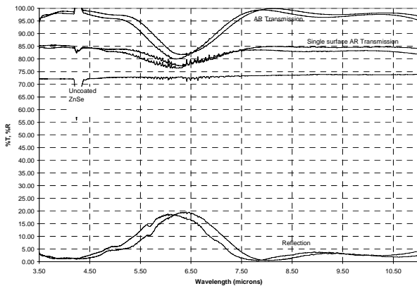
Figure 24: Measured transmission and reflection for the ZnSe 2-material design on both surfaces of a 1 mm thick ZnSe witness part.
